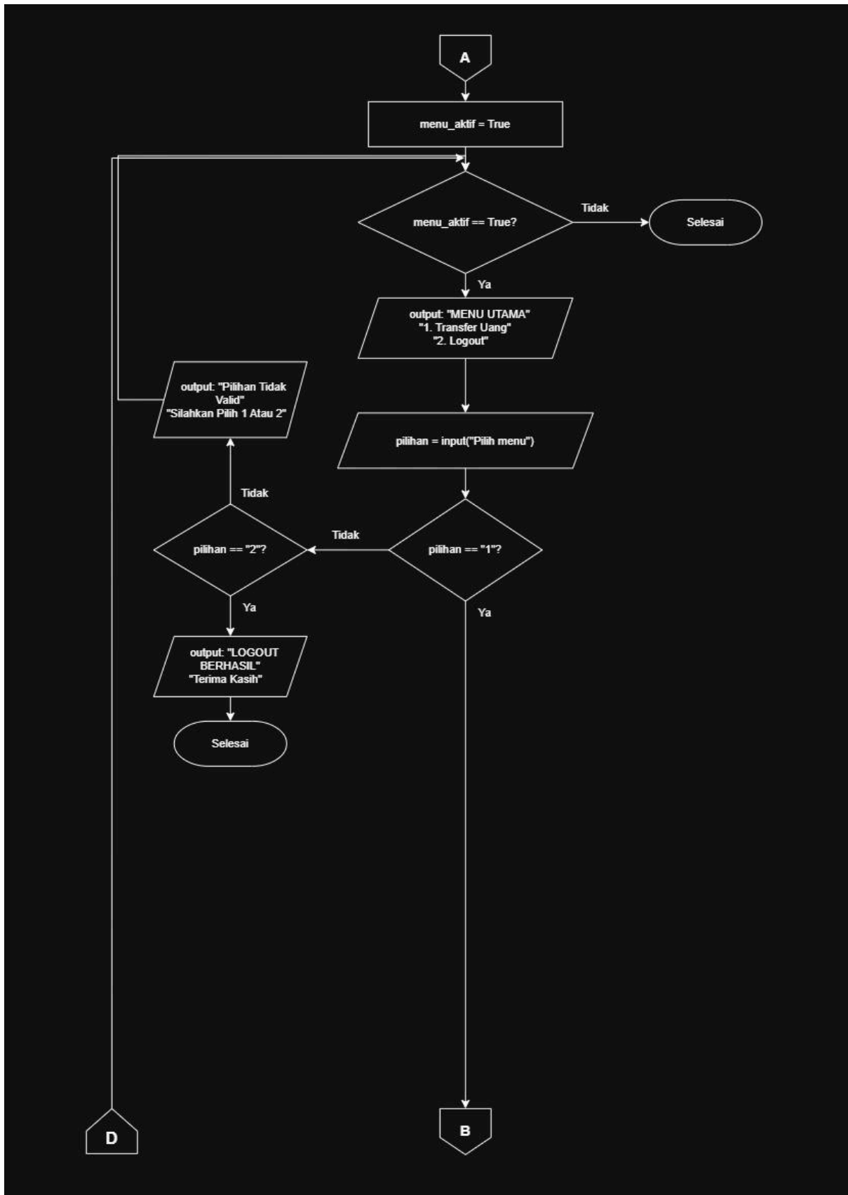
Gambar 1.2 Flowchart Halaman 2
