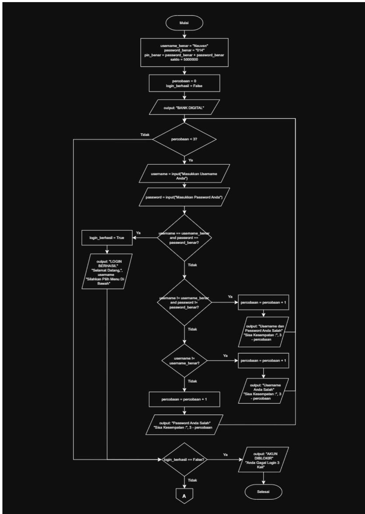
Gambar 1.1 Flowchart Halaman 1
