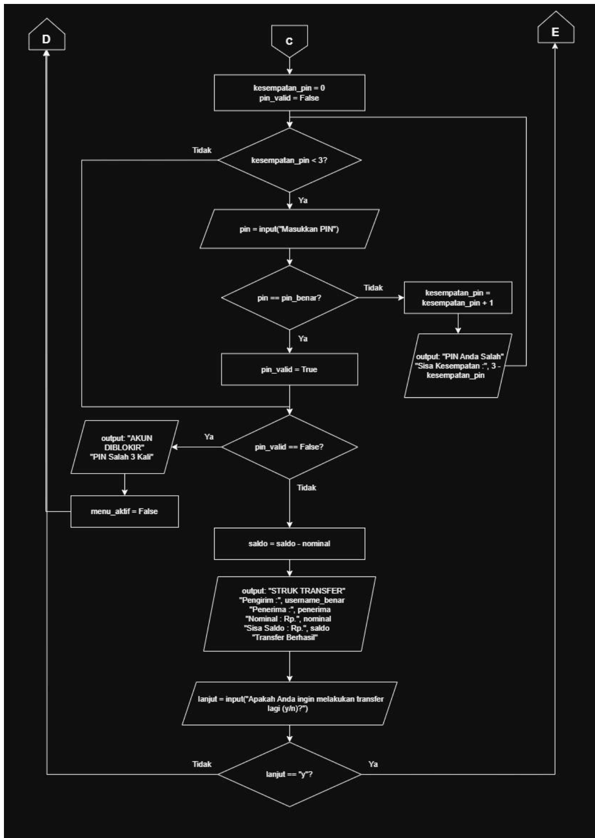
Gambar 1.4 Flowchart Halaman 4
