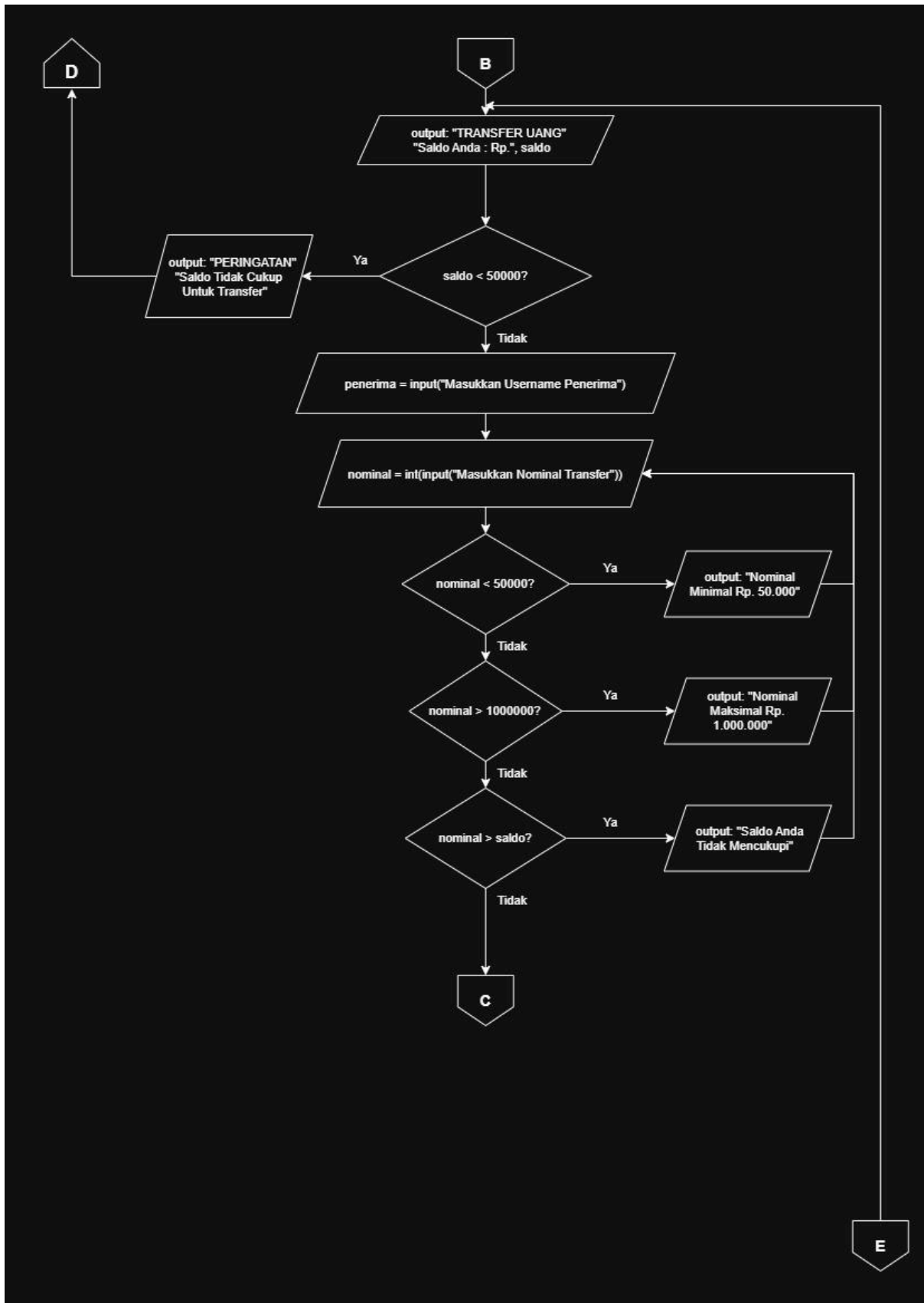
Gambar 1.3 Flowchart Halaman 3
